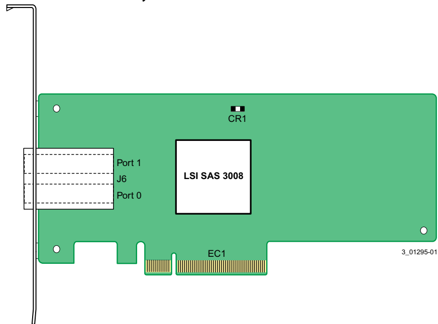
Figure 1 LSI SAS 9300-8e HBA Board Layout
