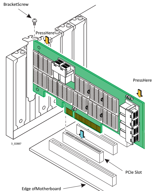
Figure 2 Installing the 12Gb/s SAS 9305-24i HBA in a PCIe Slot
