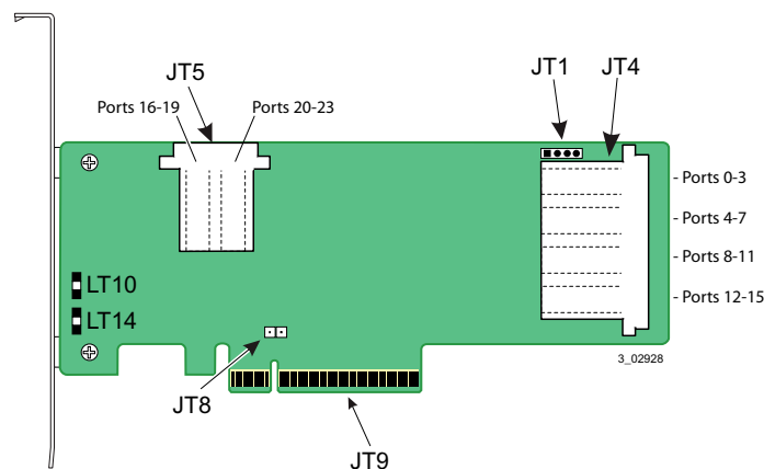
Figure 1 Avago SAS 9305-24i HBA Board Layout
