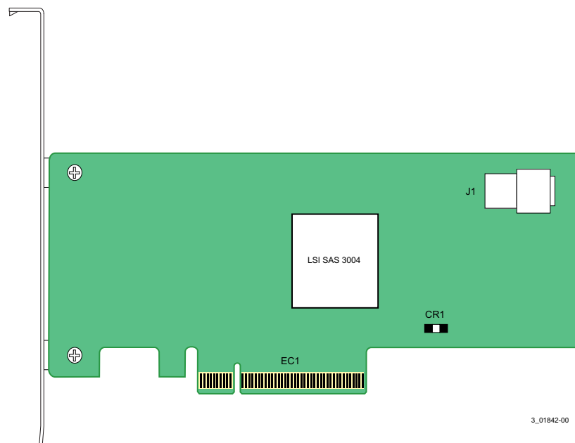
Figure 1 LSI SAS 9300-4i HBA Board Layout
