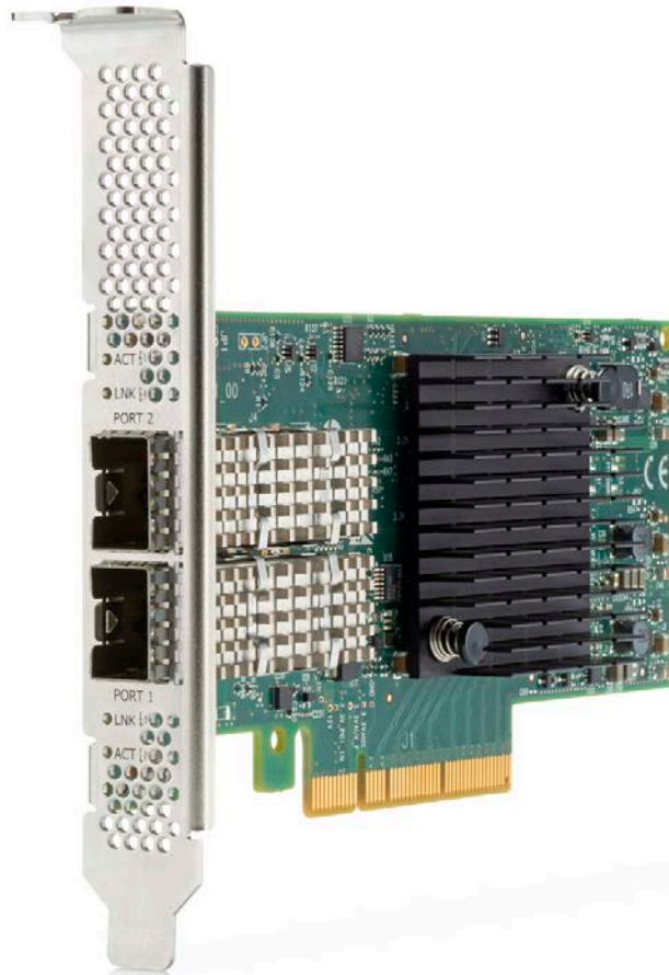
HPE Ethernet 10/25G 2-port 640SFP28 Adapter
